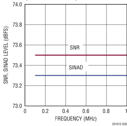
SNR, SINAD vs Input Frequency (100kHz to 1MHz)
